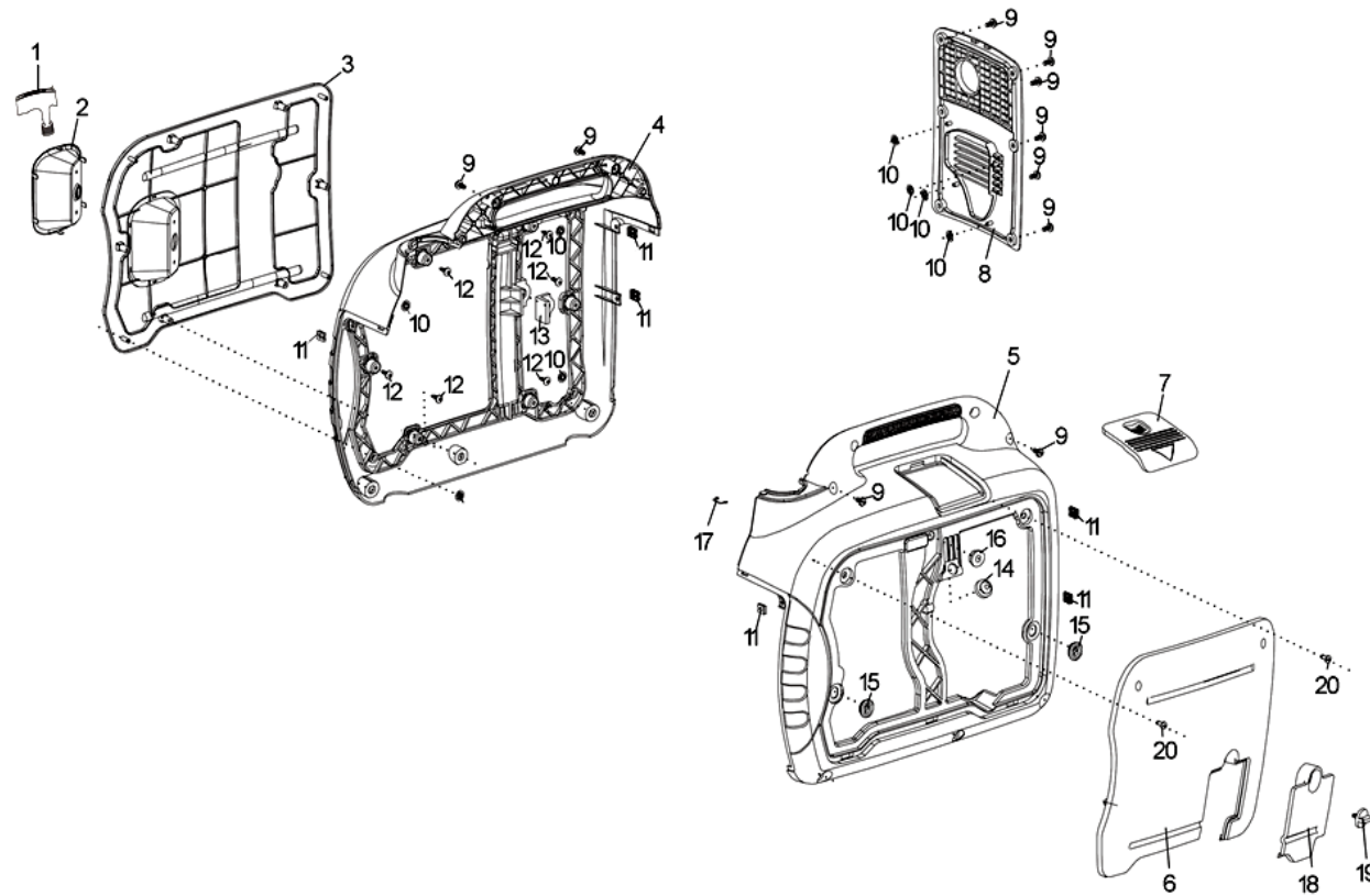
HPG1600i2 外観(APPEARANCE ASSEMBLY)2
