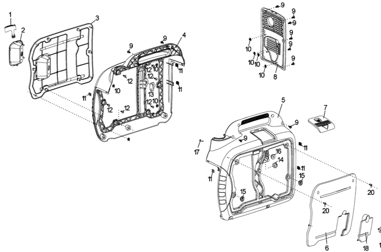
HPG1600i2 外観 (APPEARANCE ASSEMBLY) 1
